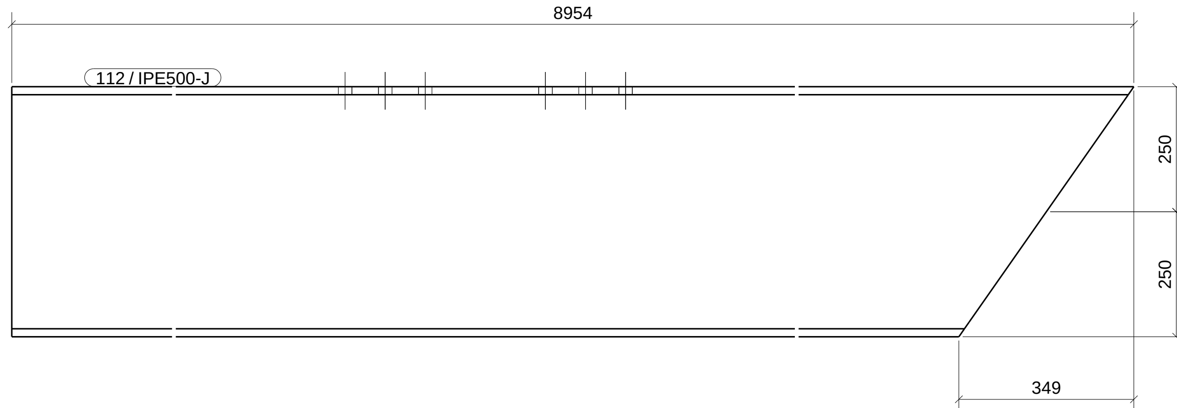
FRONT VIEW
